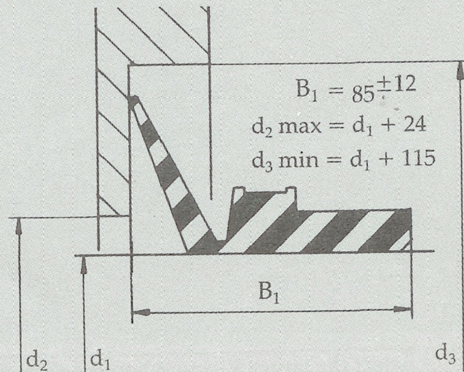
Assembly Dimensions
